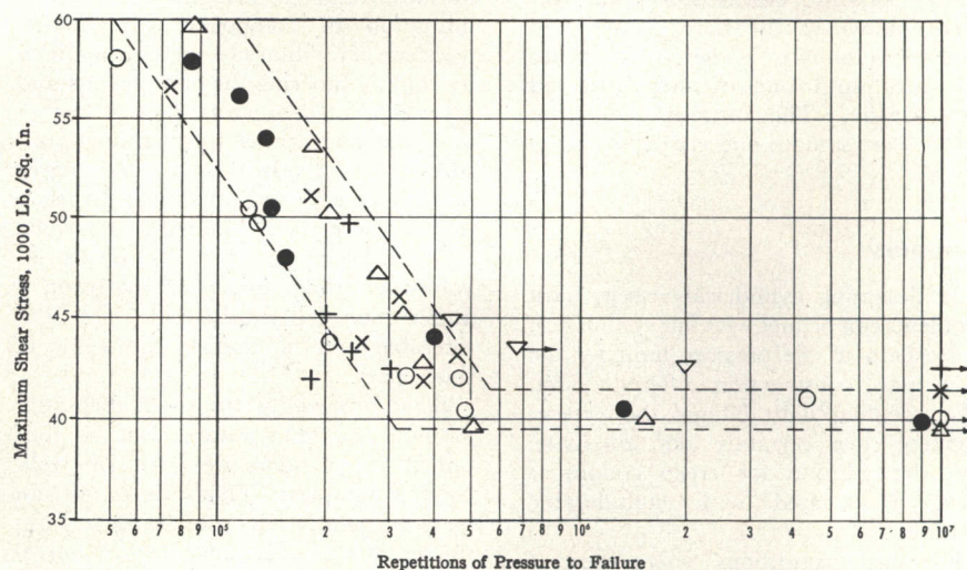
Figure 9. Fatigue of nickel-chromium-molybdenum steel cylinders (17)
